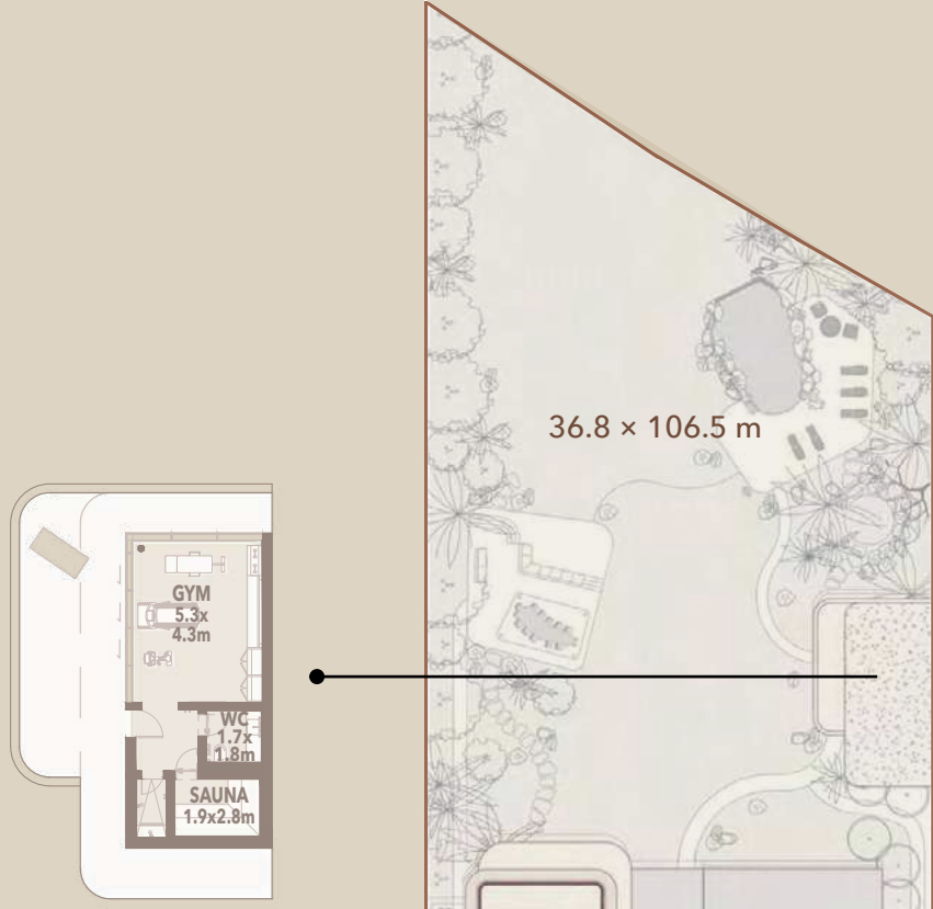
GYM PAVILION FLOOR PLAN
