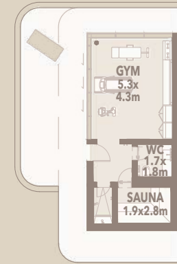
GYM PAVILION FLOOR PLAN
